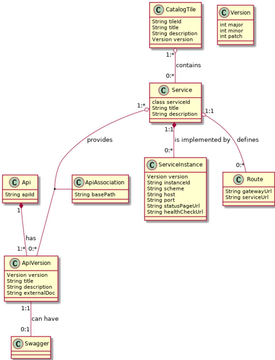
(this a UML class diagram)
